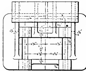
Fig. 2148. Front Elevation of Buffer Head THE GOULD TENDER-BOOK.
